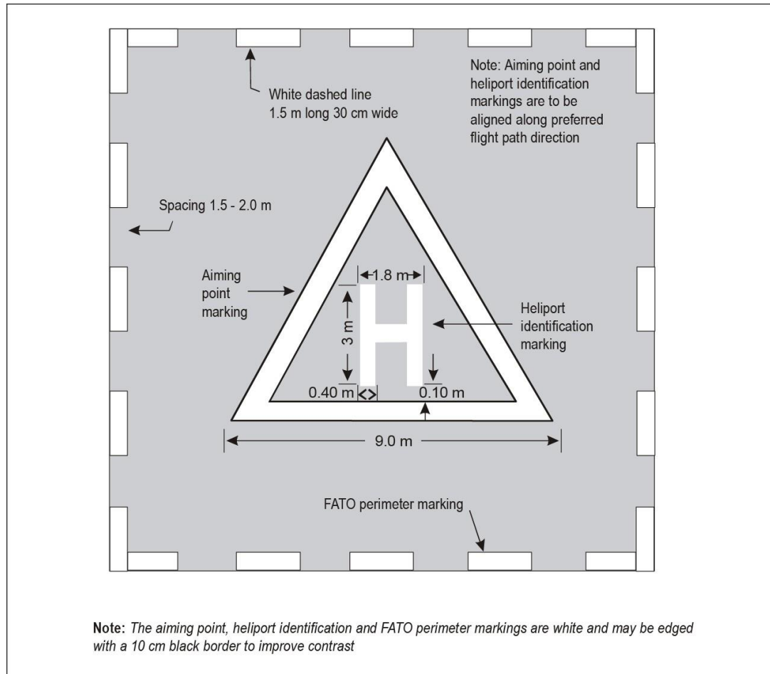
Figure 3: FATO and aiming point marking requirements (not to scale)
