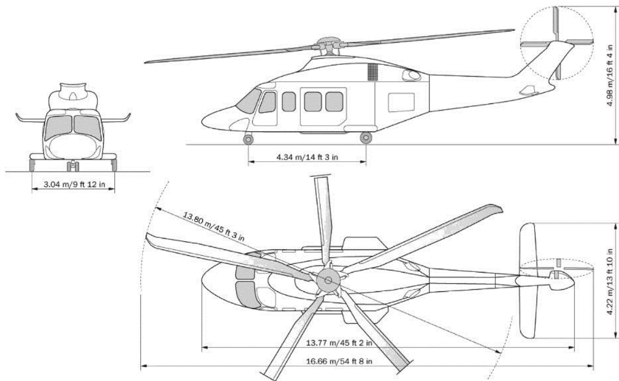
Figure 8: Dimensions of the AB139 helicopter
