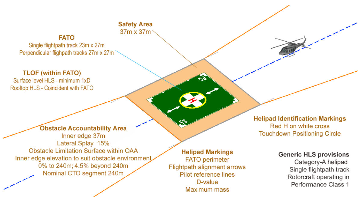
Figure 1: Layout of a generic heliport to meet design helicopter Category-A criteria (single flightpath track)
