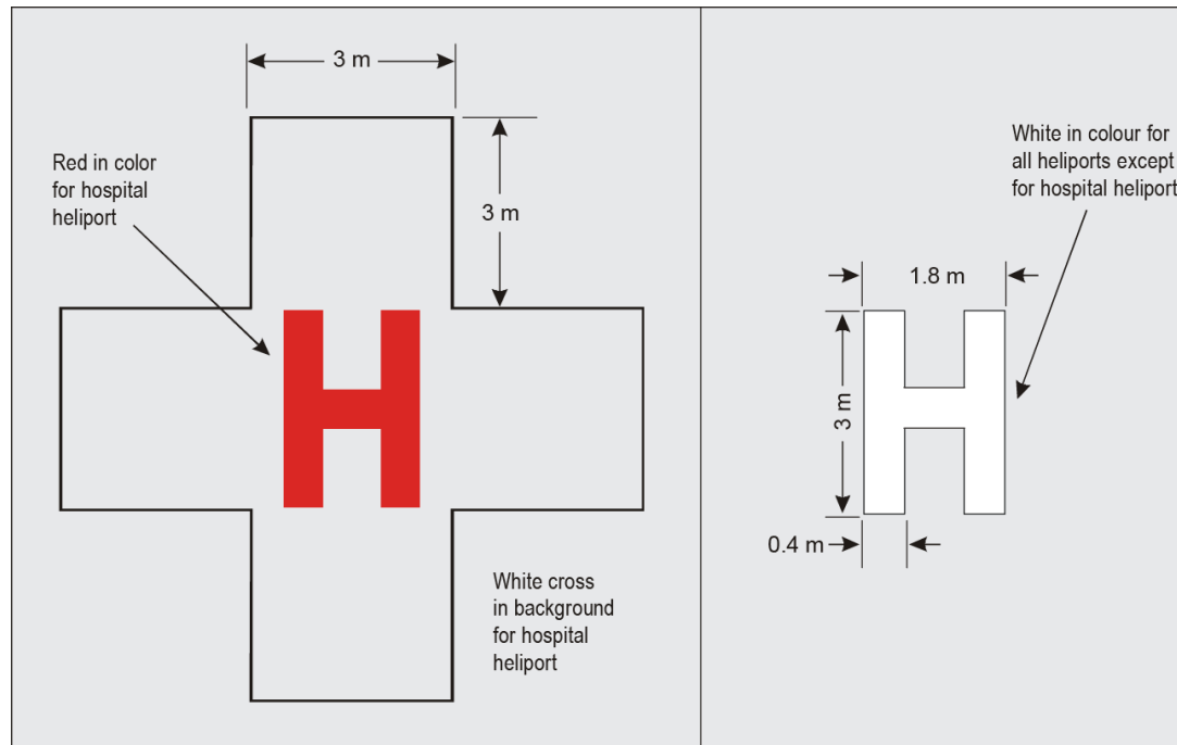
Figure 2: Hospital heliport identification marking
