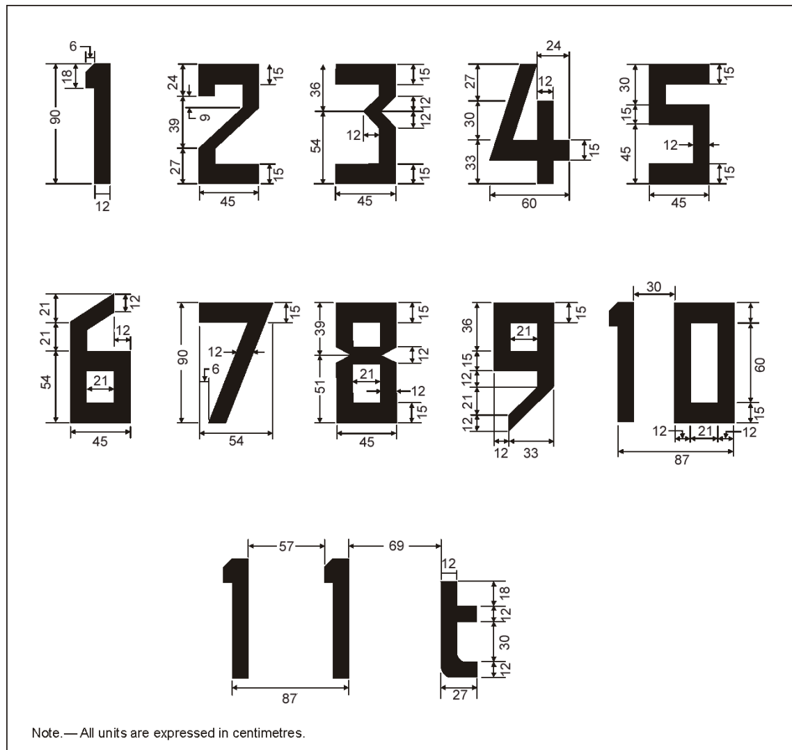
Figure 4: Form and proportion of numbers and letters for surface markings
