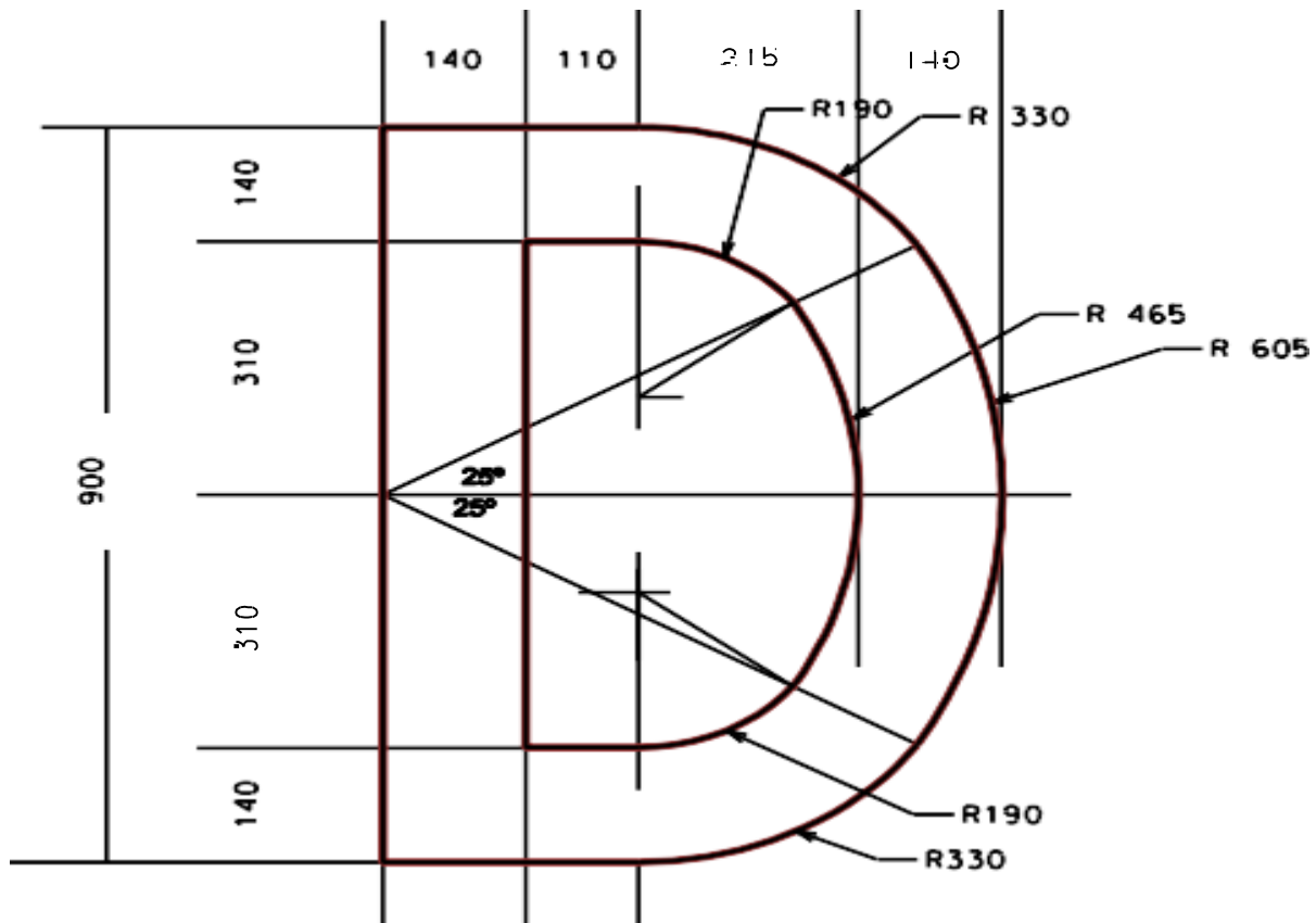
Figure 5: Form and proportion of 'D' character
